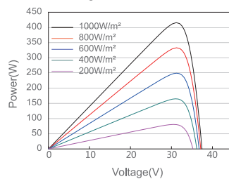
Power-Voltage Curve JAM54S31-415/GR/1000V
