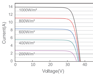
Current-Voltage Curve JAM54S31-415/GR/1000V
