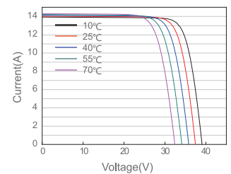
Current-Voltage Curve JAM54S31-415/GR/1000V
